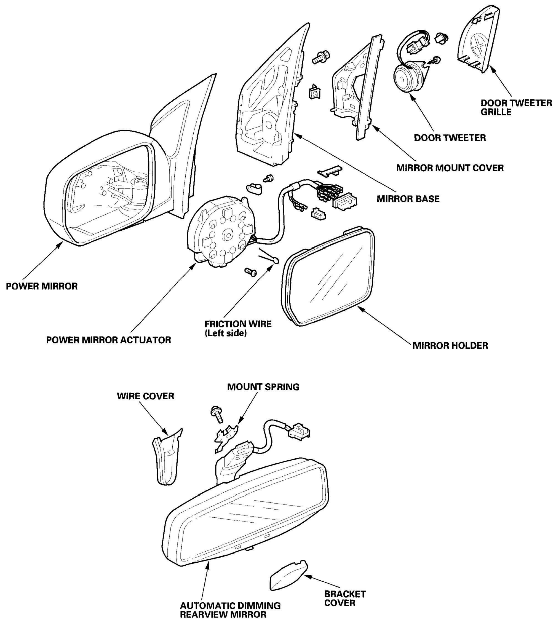
Fig. 1: Locating Mirrors Components Courtesy of AMERICAN HONDA MOTOR CO., INC.
